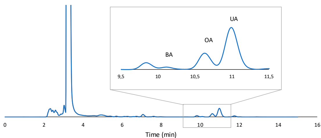
Figure S1. Illustrative HPLC chromatogram corresponding to the extraction using the NADES menthol:thymol at a molar ratio of 1:2 at 90°C (0.15 S/L ratio).
