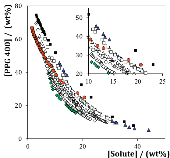
Fig. 2. Ternary phase diagrams at 25^\circ\text{C} for the systems composed of water + PPG 400 and: (■) sucrose, (▲) TES, (●) HEPES, (◆) [Ch]Cl, (◇) [Ch][Tricine] (Δ) [Ch][TES], (○) [Ch][HEPES], and (□) [Ch][MES].
