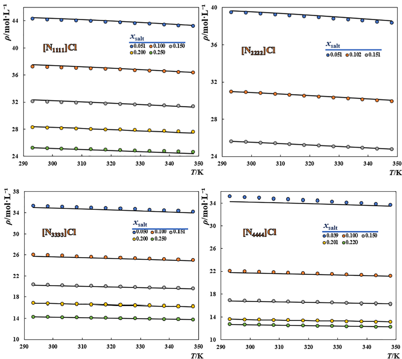
Fig. 3. Densities of aqueous solutions of symmetrical tetraalkylammonium chlorides. Symbols represent experimental data form this work while the solid lines depict the PC-SAFT results.
