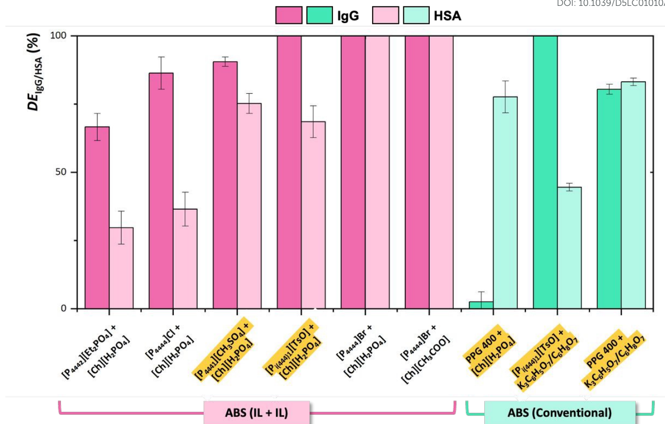
Fig. 3 Depletion efficiencies of IgG ( DE_{\text{IgG}} , %) and HSA ( DE_{\text{HSA}} , %) obtained for IL-IL ABS (pink) composed of 30 or 40 wt% phosphonium-based IL + 35 wt% cholinium-based IL + 33 or 23 wt% PBS + 2 wt% human serum, and for conventional ABS (green) composed of 30 wt% [P_{i(444)1}][\text{TsO}] or PPG 400 + 35 wt% [\text{Ch}][\text{H}_2\text{PO}_4] or \text{K}_3\text{C}_6\text{H}_5\text{O}_7/\text{C}_6\text{H}_8\text{O}_7 + 33 wt% phosphate buffered saline solution (PBS) + 2 wt% human serum. Within each ABS type, darker bars correspond to IgG and lighter bars to HSA. The systems selected for subsequent HER2 extraction experiments are highlighted in yellow. Error bars represent standard deviation ( n=3 ).
