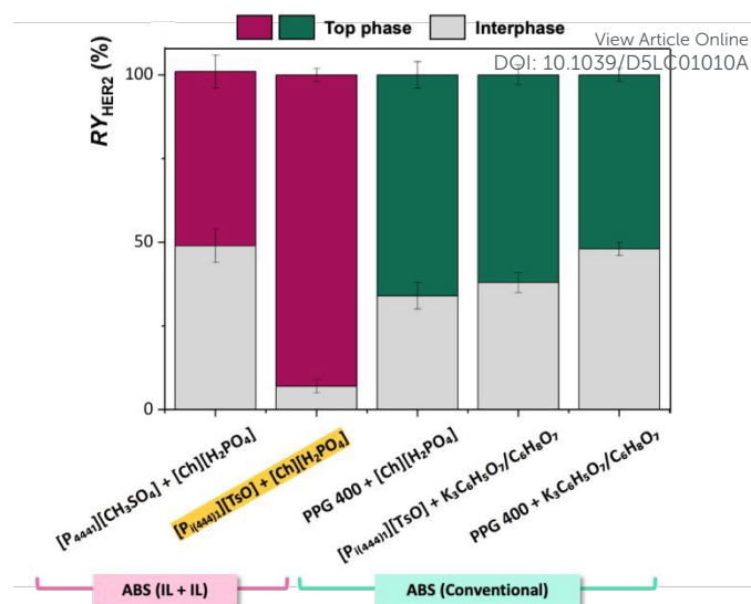
Fig. 4 Recovery yields of HER2 ( RY_{HER2} , %) in IL-IL ABS (pink) composed of 30 wt% phosphonium-based IL + 35 wt% cholinium-based IL + 33 wt% PBS + 2 wt% HER2 spiked human serum ( 15 \text{ ng}\cdot\text{mL}^{-1} ), and of conventional ABS (green) composed of 30 wt% [P_{i(444)}][TsO] or PPG 400 + 35 wt% [Ch][H_2PO_4] or K_3C_6H_5O_7/C_6H_8O_7 + 33 wt% PBS + 2 wt% HER2 spiked human serum ( 15 \text{ ng}\cdot\text{mL}^{-1} ). Each bar is stacked to indicate the fraction of HER2 recovered in the top phase (coloured segment) and interphase (grey segment). The best-performing system for HER2 extraction is highlighted in yellow. Error bars represent standard deviation ( n=3 ).
