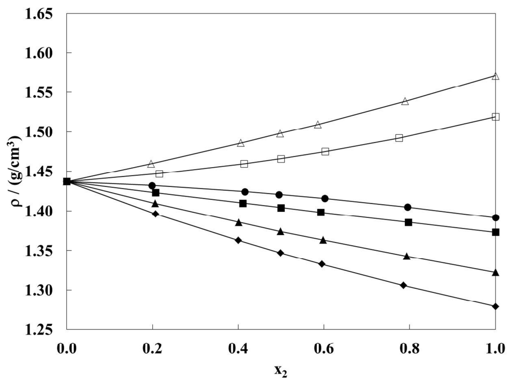
Figure S1. Experimental density data at 298.15 K of the binary systems composed of [\text{C}_4\text{mim}][\text{NTf}_2] (1) + [\text{C}_n\text{mim}][\text{NTf}_2] (2) (symbols and lines): \triangle , [\text{C}_1\text{mim}][\text{NTf}_2] ; \square , [\text{C}_2\text{mim}][\text{NTf}_2] ; \bullet , [\text{C}_5\text{mim}][\text{NTf}_2] ; \blacksquare , [\text{C}_6\text{mim}][\text{NTf}_2] ; \blacktriangle , [\text{C}_8\text{mim}][\text{NTf}_2] ; \blacklozenge , [\text{C}_{10}\text{mim}][\text{NTf}_2] .
