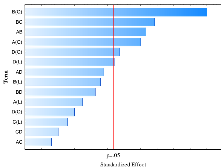
Fig. S1. Pareto chart for standardized effects for recovery oil. A = P (bar); B = m_c (g); C = N_c (number of compressions); D = t_c (min).
