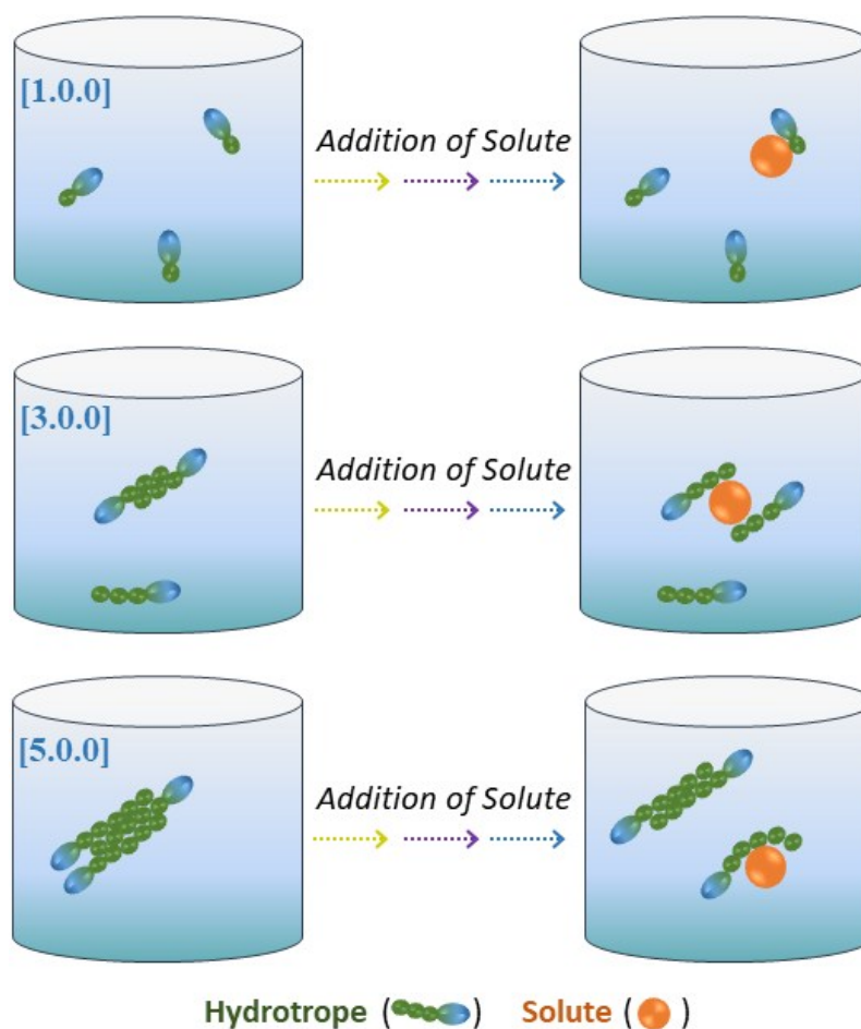
Figure S5. Schematic illustration of the hydrotropy mechanism, evidencing the main findings in this work. In the first case, apolarity of the hydrotrophe is small and the driving force for aggregation is low; in the second case, apolarity of the hydrotrophe is equal to that of the solute and the driving force for aggregation is maximized, resulting in more hydrotrophe molecules aggregated around the solute; in the third case, apolarity of the hydrotrophe is greater than that of the solute and, thus, driving force for hydrotrophe-hydrotrophe aggregation is larger than that of hydrotrophe-solute aggregation.
