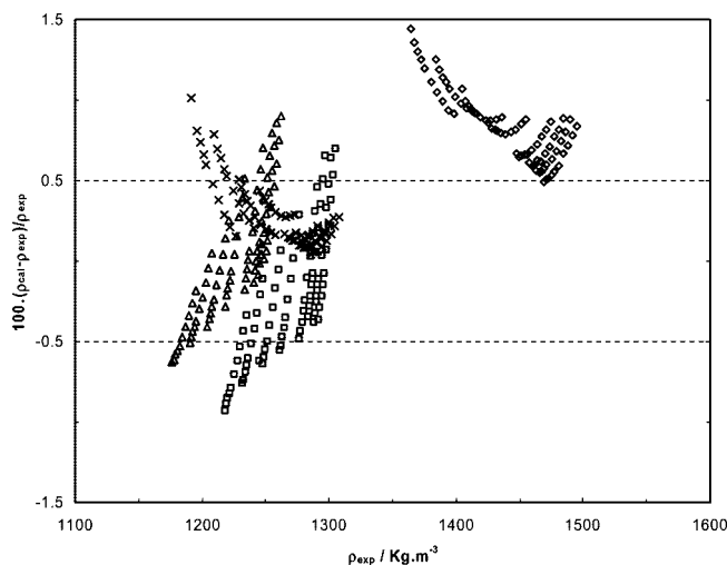
Figure 7. Relative deviations between the experimental and calculated density using eq 11 as a function of experimental density of ionic liquids: □, [C_2mim][MeSO_4] ; △, [C_2mim][EtSO_4] ; ◇, [C_2eim][Tf_2N] ; ×, [C_{10}mim][Tf_2N] .
