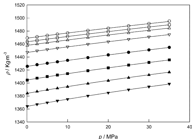
Figure 3. Isotherms of the density, \rho , for [C 2 eim][Tf 2 N]. The symbols refer to the experimental data: \circ , 293.15 K; \square , 298.15 K; \Delta , 303.15 K; \nabla , 313.15 K; \bullet , 333.15 K; \blacksquare , 353.15 K; \blacktriangle , 373.15 K; \blacktriangledown , 393.15 K. The curves are calculated with the Tait equation, eq 1.
