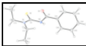
Fig. 1. A view of (I) with displacement ellipsoids drawn at the 30% probability level.
