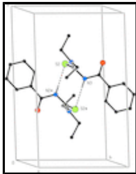
Fig. 2. A view of the R^2_2(8) dimer lying across the centre-of symmetry at (0.5,0.5,0.5). Atoms marked with an asterisk,*, are in the molecule at (1-x,1-y,1-z). Hydrogen atoms not involved in the hydrogen bonding are omitted for the sake of clarity.
